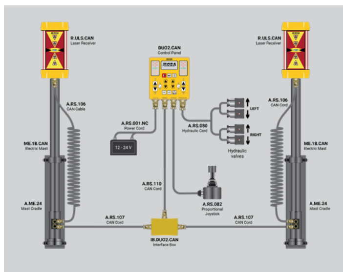
RS.037 Typical dual receiving system
